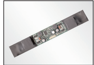
C Backlight Inverter Board (LD 2771) CAUTION: High Voltage The heat shrink tubing is used for your protection.
