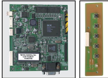
B TFT Controller Board with On-Screen Display (OSD) Board (VNS-AV-084VGATTL-00)
